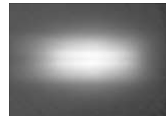
Elliptical orthogonal Optic 10397 "Note the dark line caused by the gap in the chips"
